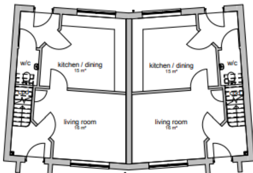
3 bedroom House
