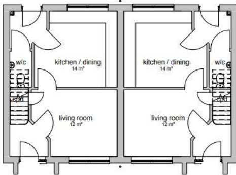
2 bedroom House
